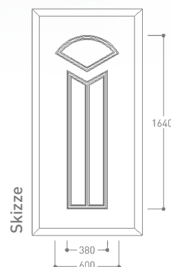
Detail Garant 8 Ornamentrahmen
